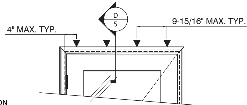
X HEAD EXTERIOR VIEW
