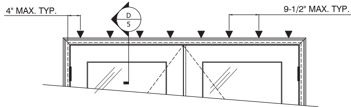
XX HEAD EXTERIOR VIEW
